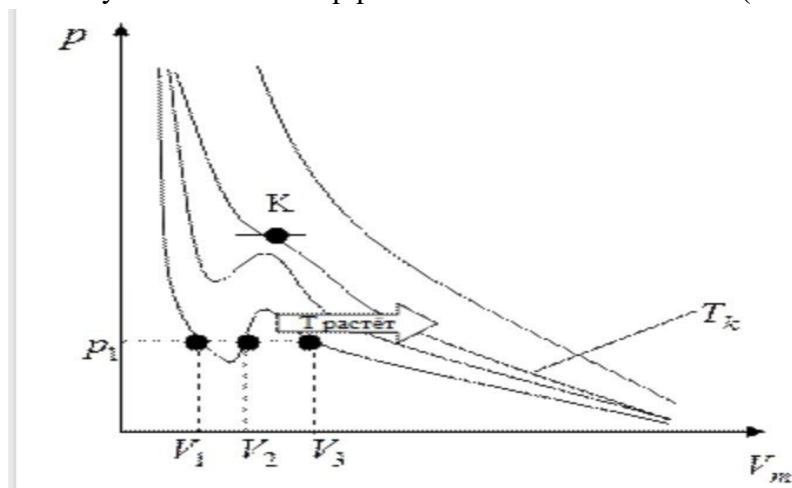
1-rasm. Real gazlar holatining Van-Der-Vaals izotermalari.
