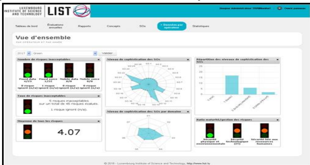
Figure 2. Screenshots of TISRIMonitor, the NRA data platform.
