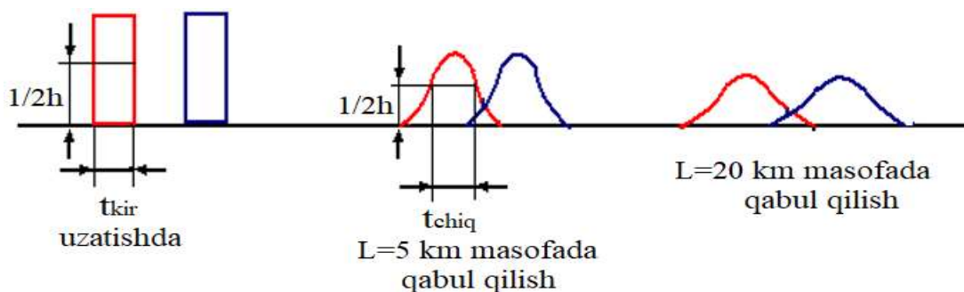
Fig. 1. Expansion of pulses due to dispersion.
