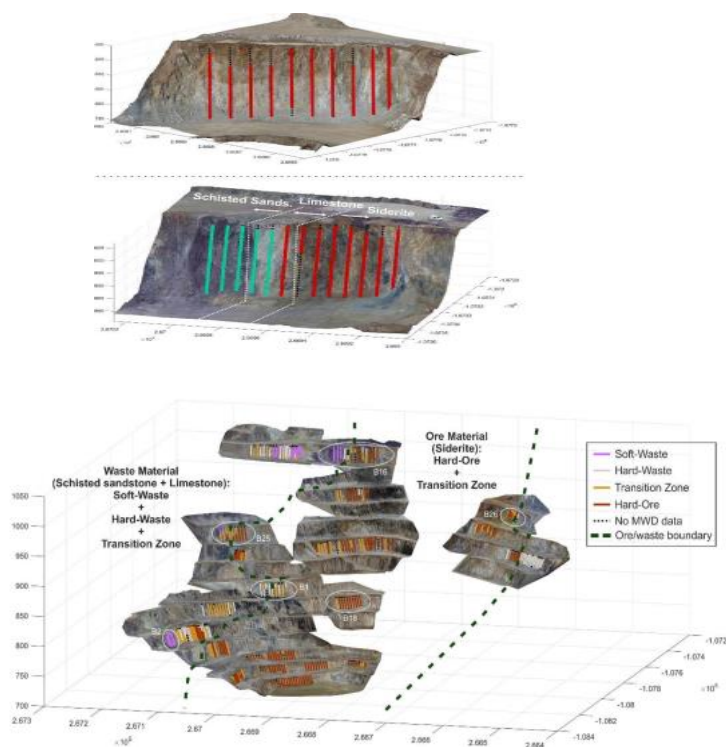
Picture1. Determining the layout of detonators in the mine field in accordance with the parameters of the technical indicators of the open mine during the drilling and blasting processes in the open mine.
