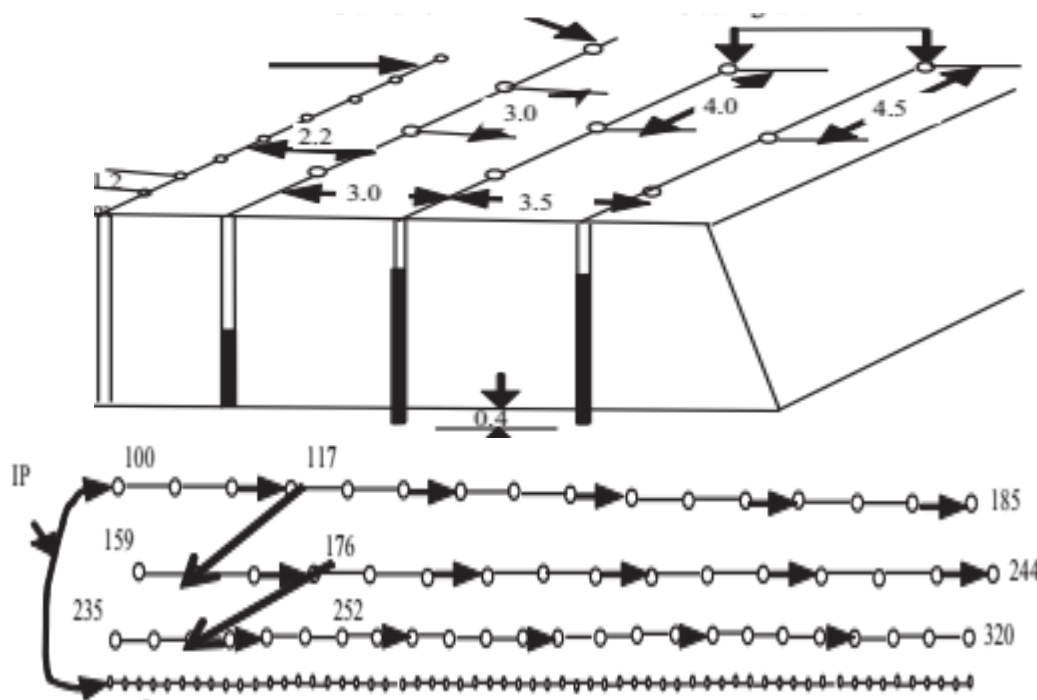
Picture 2. Mine blasting design and explosion sequence in charging.
