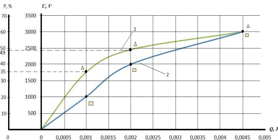
Figure 2. Diagram of voltage magnitude variation from the time of electric current pulses for tomatoes
