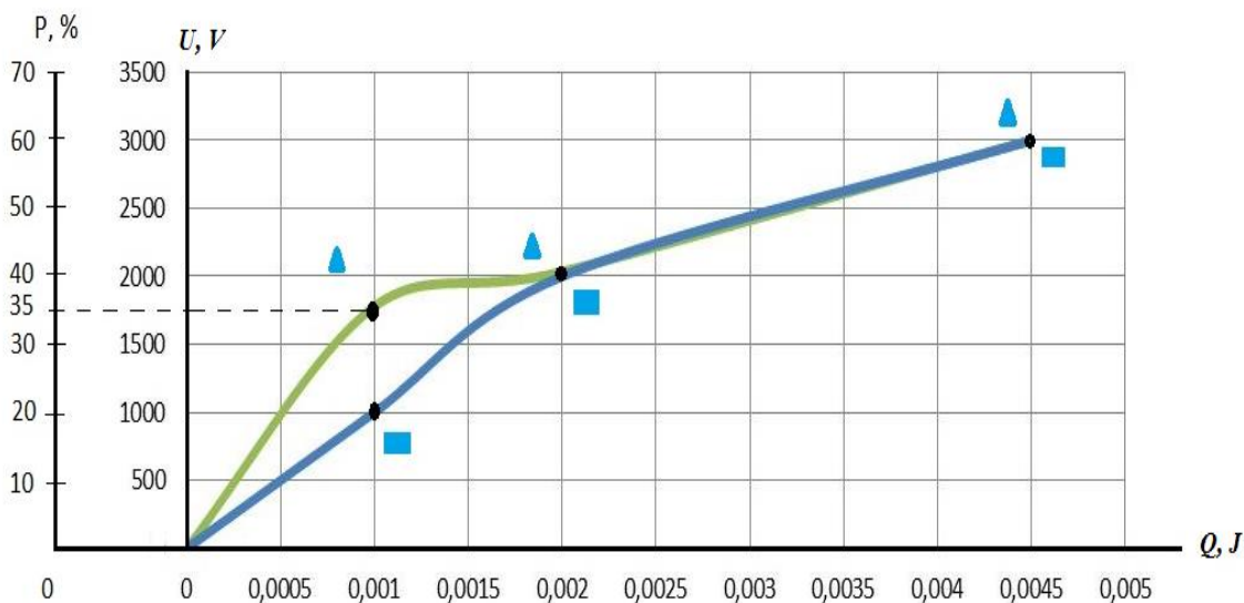
Figure 3. Variation of voltage magnitude from pulse time by electric pulse current discharge for cucumbers
