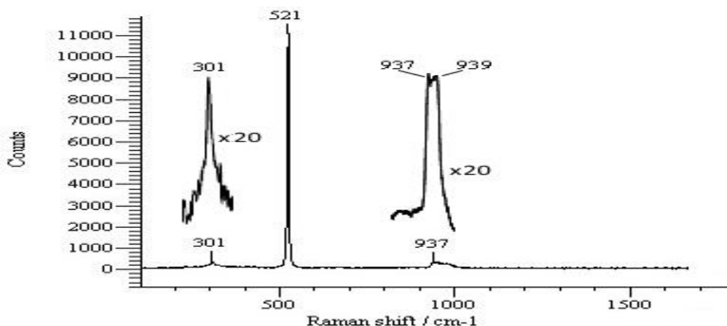
Fig. 5. Raman spectra of Si(111) with a SiO 2 film 100 Å thick.
