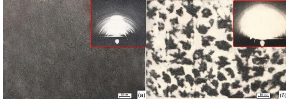
Fig. 1. SEM images and RHEED patterns (insets) for the Si/Cu(100) surface before (a) and after (b) implantation with ions with energy E = 1.0 \text{ keV} at a dose of 6 \times 10^{15} \text{ sm}^{-2} [3-4].
