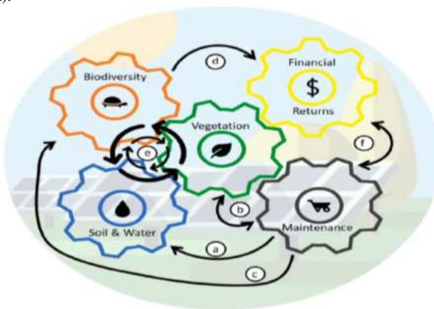
Fig. 2. Conceptual model of components and interactions that influence land condition in agrivoltaic systems. Five major components are summarized through their interactions (represented by a – f and described in the text): Biodiversity (wildlife habitat, species diversity, refugia and cover, pollinator and predators, and ecosystem services); Soil and Water (run-off,
