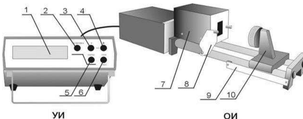
Fig. 5 . Schematic diagram of the installation. 1- Indicator, 2- Button "Setting", 3 and 4- buttons (+, -), 5-reset, 6-start and stop, 7- Counter block, 8- Curtain, 9-line with a scale, 10-source Alpha particle [3].
